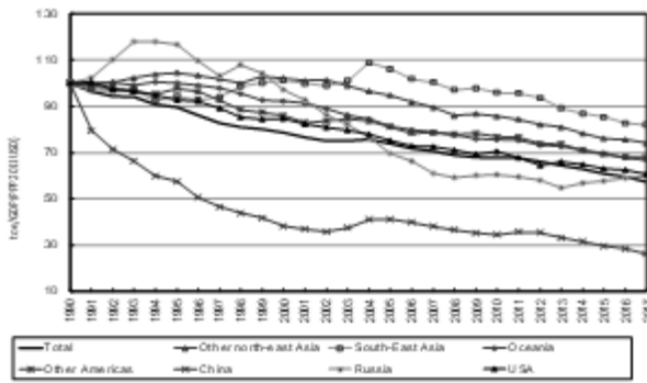
Figure 2.18 • Final energy intensity by region, 1990-2017
