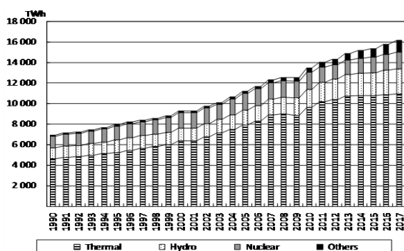
Figure 2.12 • Power generation by type, 1990-2017
