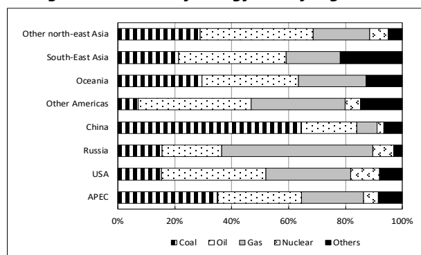
Figure 2.7 • Primary energy mix by region, 2017
