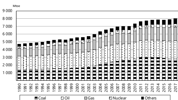
Figure 2.5 • Total primary energy supply, 1990-2017
