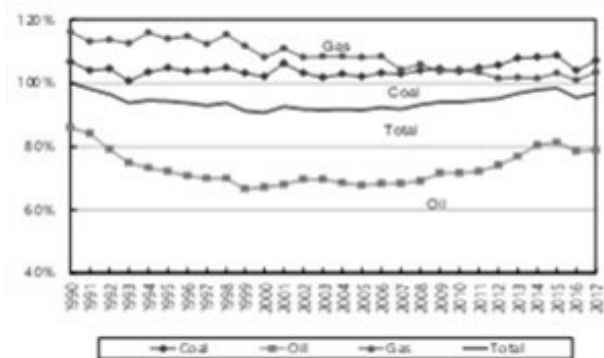
Figure 2.10 • APEC energy self-sufficiency, 1990-2017
