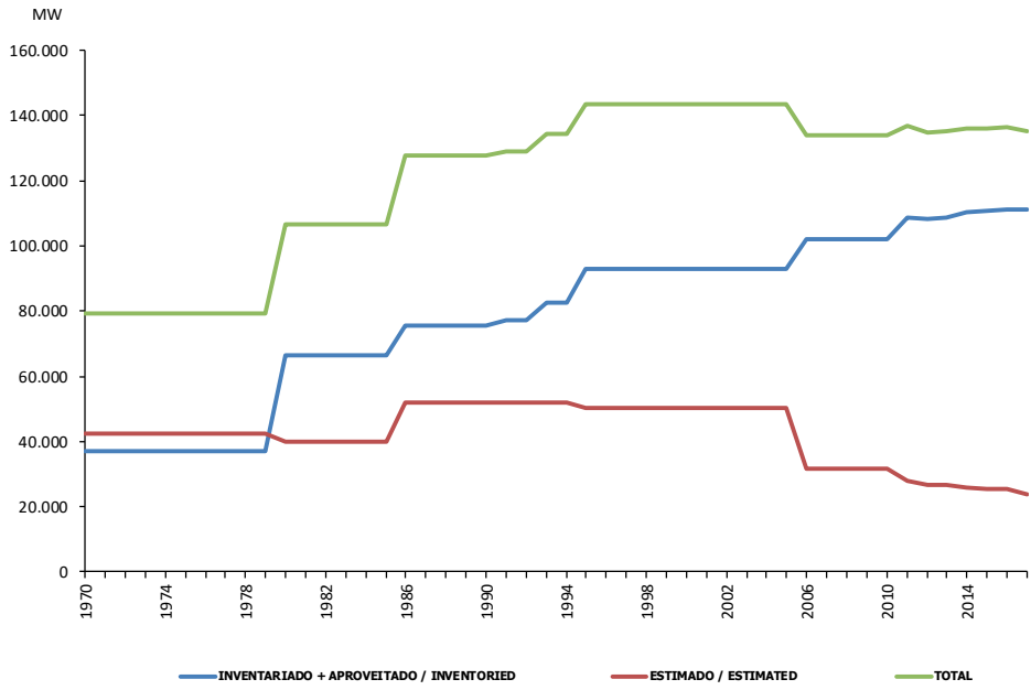
Chart 6.3 – Hydraulic Potential
