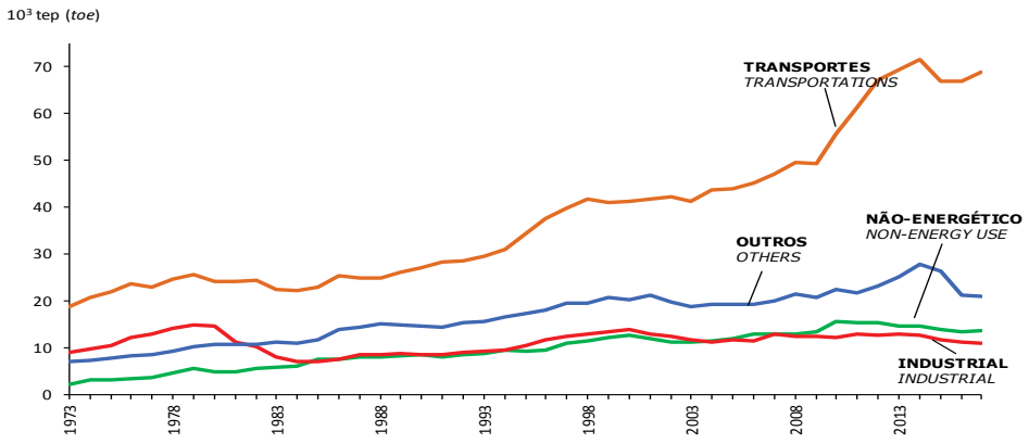
Chart 2.6 – Total Consumption of Oil Products and Natural Gas Products
