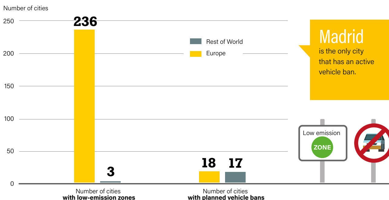
FIGURE 12. Number of Cities with Low-Emission Zones and Planned Vehicle Bans, Europe and Rest of World, As of Mid-2019
