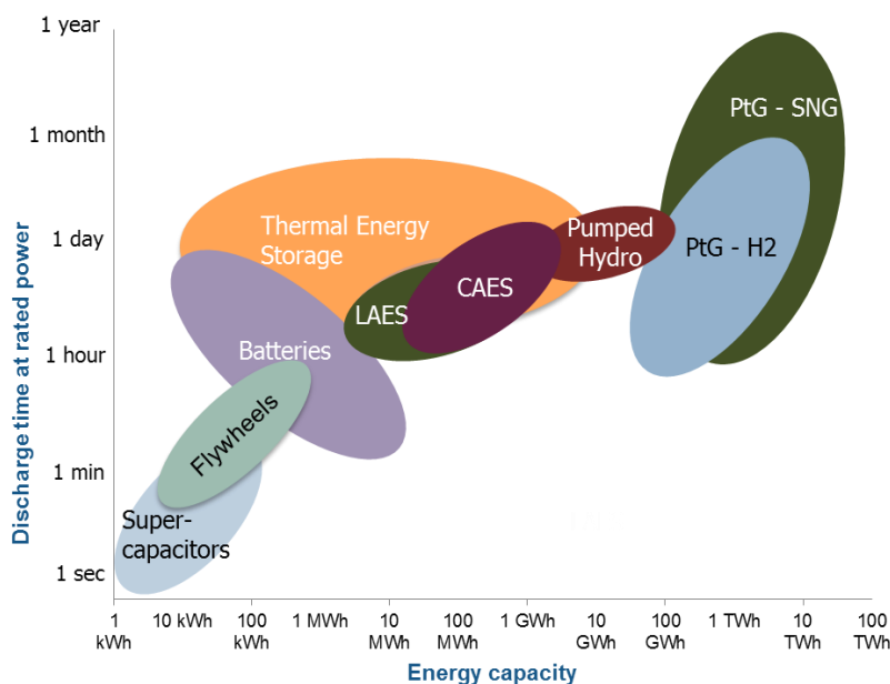
FIGURE 21: MAPPING STORAGE TECHNOLOGIES ACCORDING TO PERFORMANCE CHARACTERISTICS
