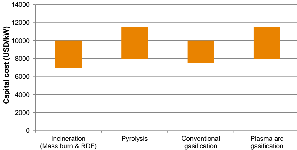
FIGURE 13: CAPITAL COSTS FOR THERMAL WTE POWER GENERATION TECHNOLOGIES IN THE UNITED STATES (15 MW OUTPUT)
