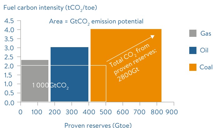
FIGURE 7: CLIMATE CHANGE CHALLENGE 19
