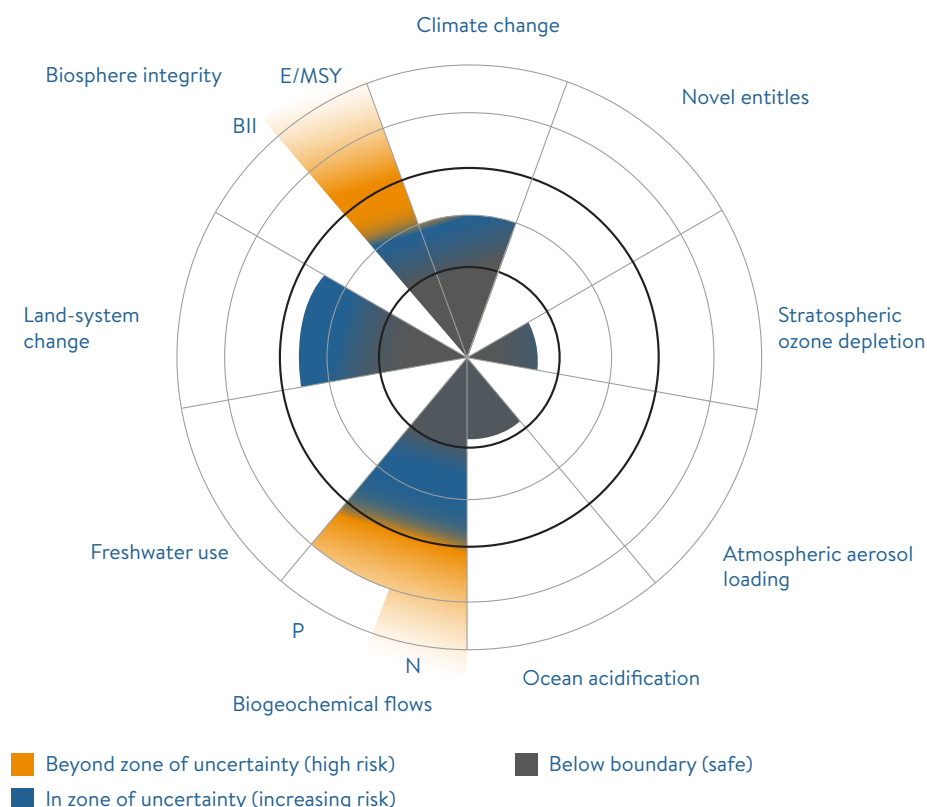
FIGURE 4: PLANETARY BOUNDARIES
