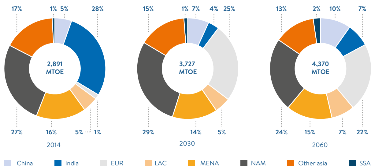
FIGURE 44: HARD ROCK GAS IN TPES BY REGION (MTOE)
