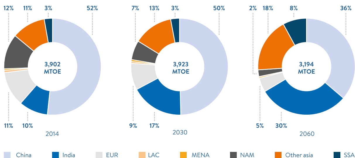
FIGURE 42: HARD ROCK COAL IN TPES BY REGION (MTOE)
