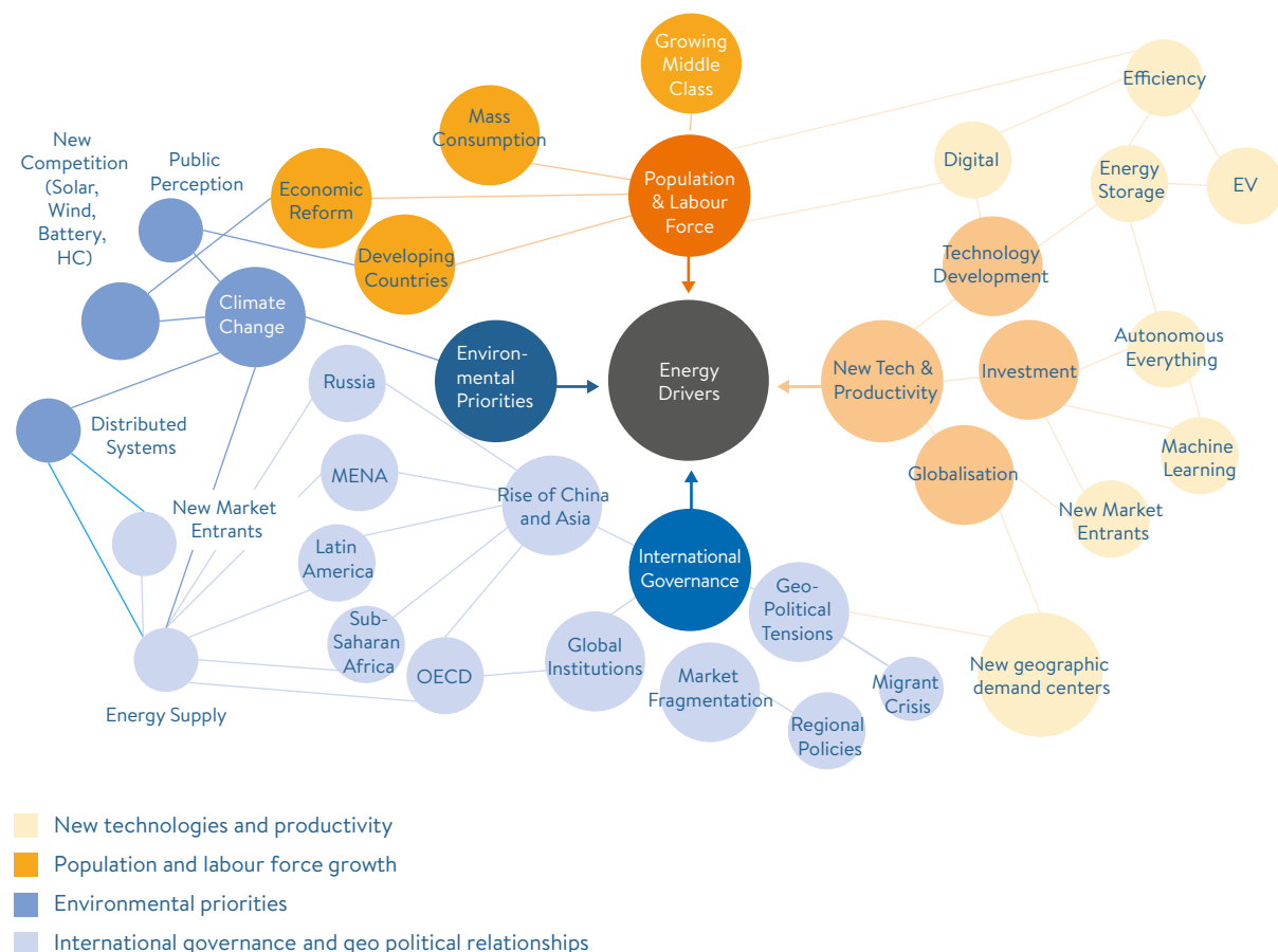
FIGURE 1: FACTORS THAT SHAPED WORLD ENERGY
